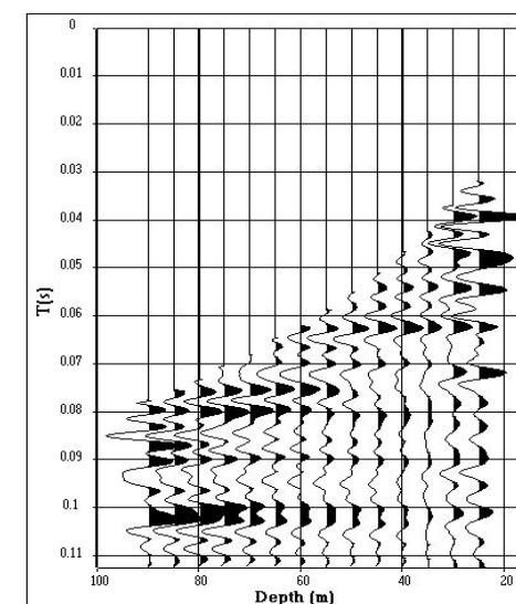
VSP : Up going waves after deconvolution
