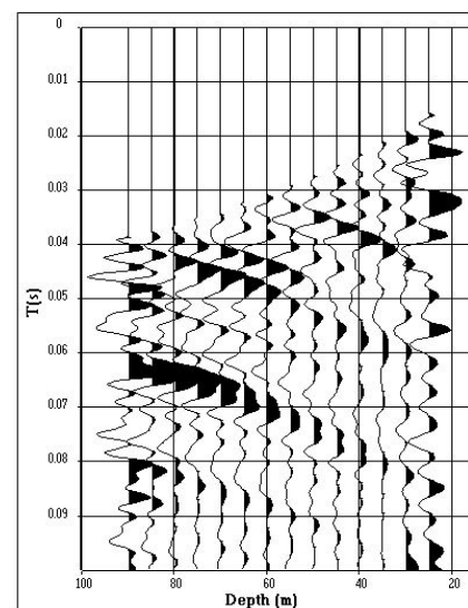
VSP : Up going waves after amplitude recovery
