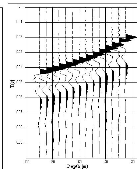
VSP : Down going waves after amplitude recovery
