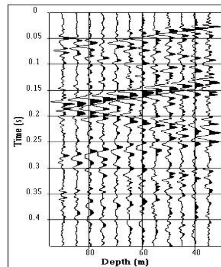
VSP with an hydrophone
